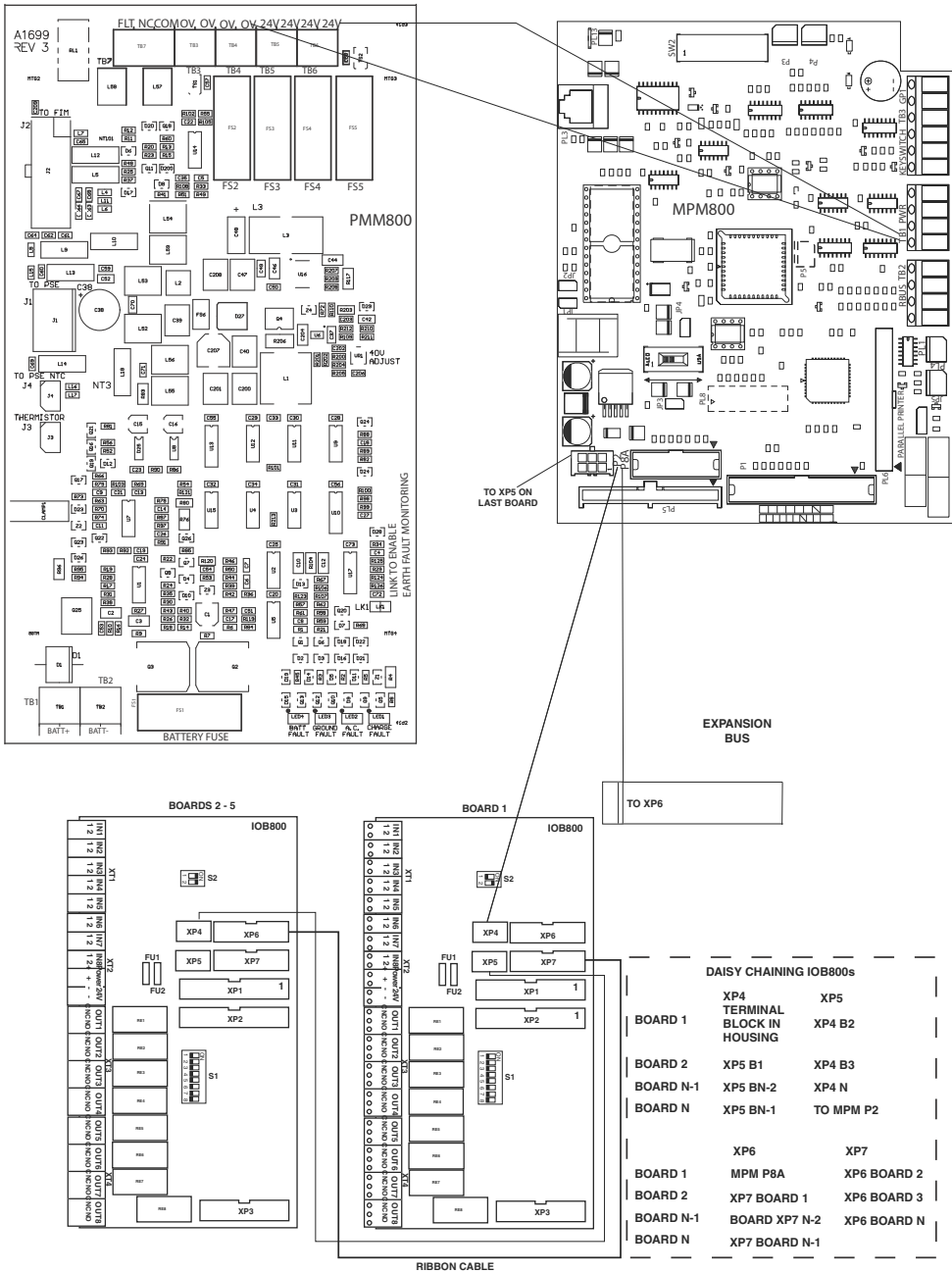
Fig. 3: IOB XBus Connections Details
