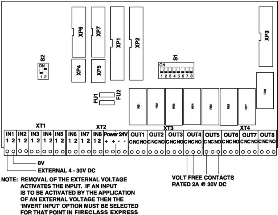
Fig. 2: IOB800 Configuration Details
