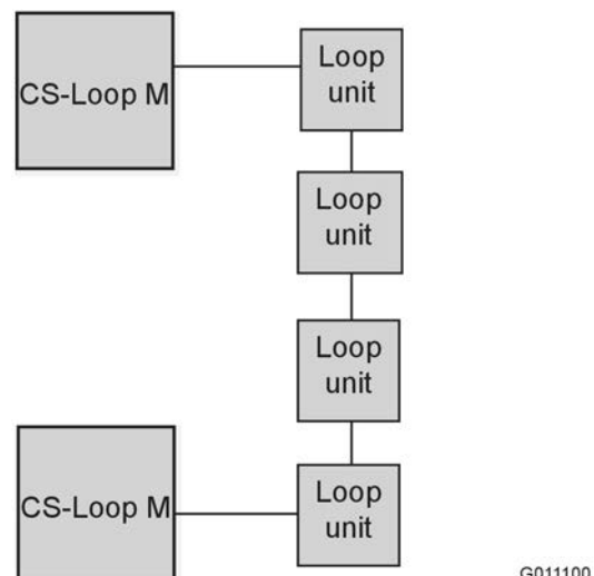
Figure 2. Example of a redundant loop-line configuration with two CS-Loop M H modules
