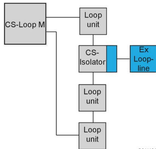
Figure 1. Example of a normal loop-line configuration
