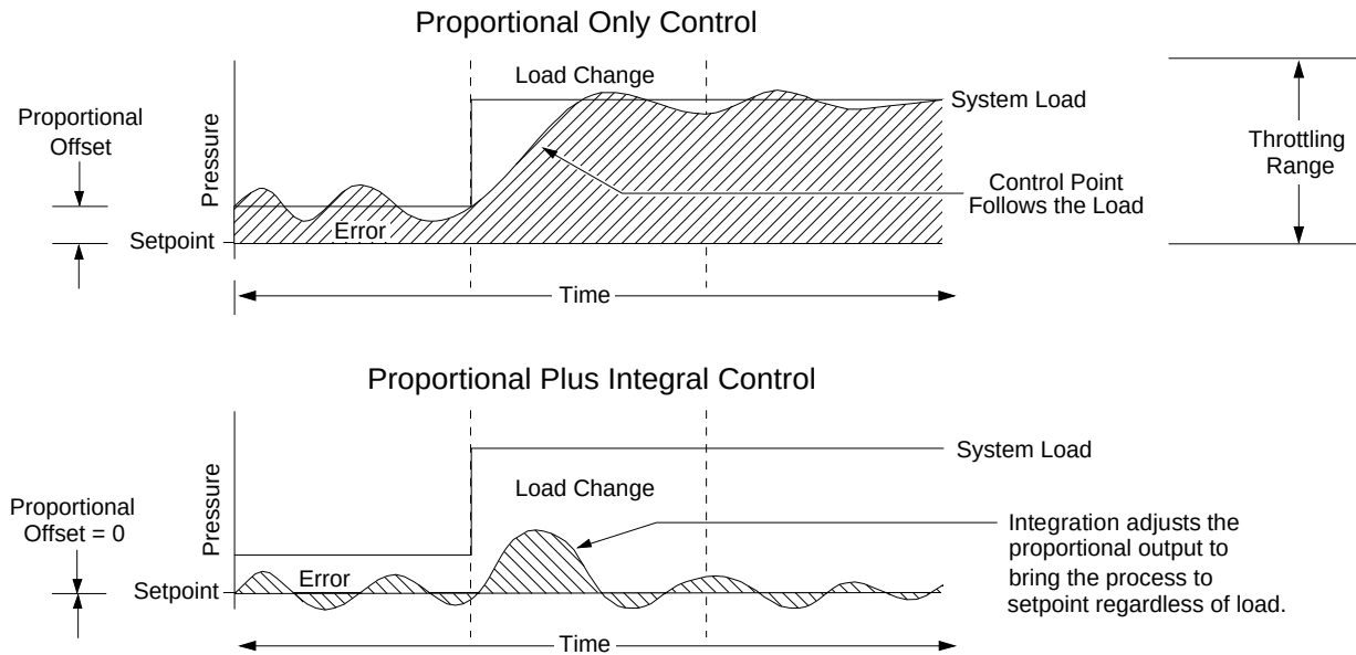
Figure 4: Operation of Proportional Only vs. Proportional Plus Integral Control
