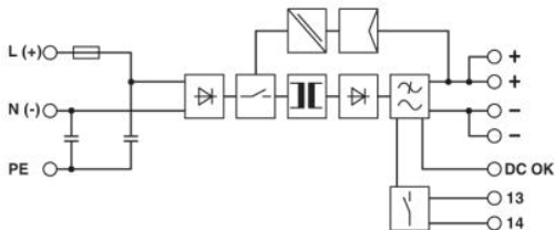
Block diagram
